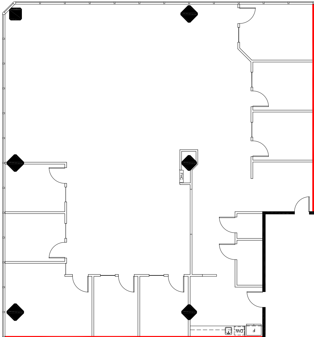
KEY PLAN
