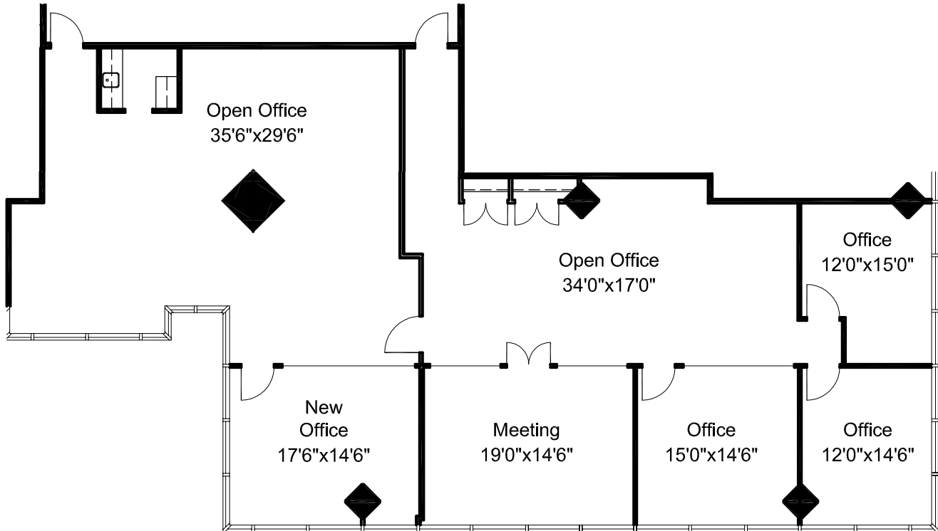
KEYPLAN
