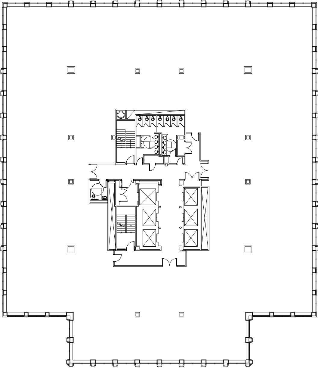
FLOOR PLAN
